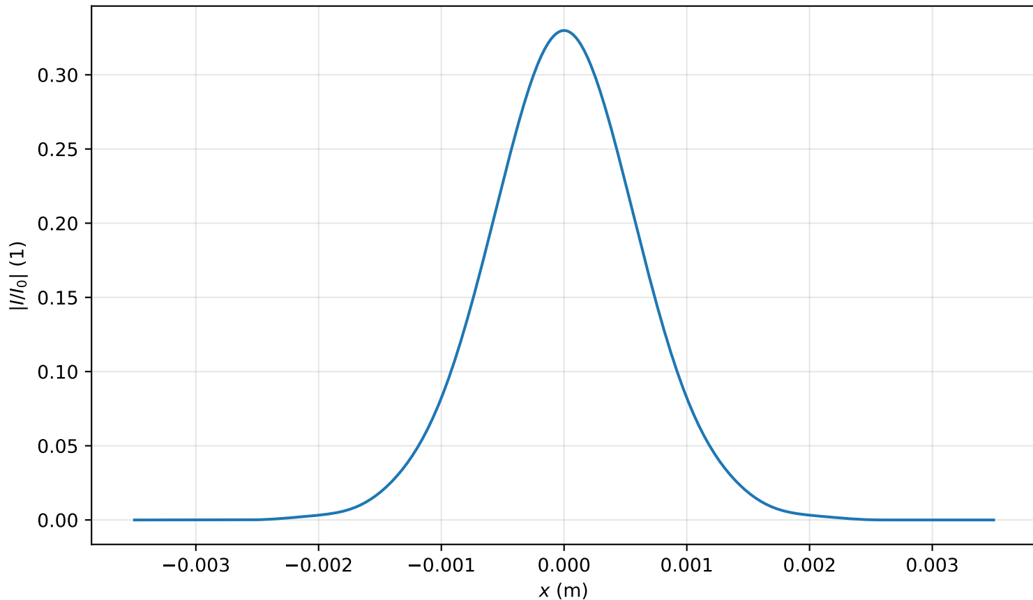
Intensity profile I(x, y = 0, z = 3.981m)/I_0 , P_{in}=0.4P_{cr} , artificial time
